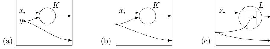
Figure 1: Graph (a) represents the term (\langle x \rangle \otimes \langle y \rangle) \cdot K \otimes \langle y \rangle which has arity 0 \rightarrow 2 . Graph (b) represents (y)((\langle x \rangle \otimes \langle y \rangle) \cdot K \otimes \langle y \rangle) : 1 \rightarrow 2 , in which the wire formerly marked y becomes part of the left interface. Graph (c) represents (y)(\langle x \rangle \cdot L(\langle y \rangle) \otimes \langle y \rangle) and illustrates a wire crossing a control boundary through the use of the abstracted name y . In all examples K : () \rightarrow (2, 1) and L : ((0, 1)) \rightarrow (1, 1) .
