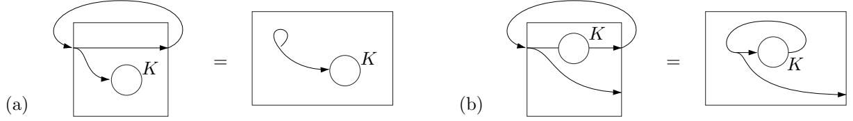
Figure 8: Two cases of reflexion in reflexive molecular forms. (a) In reflecting \uparrow (x)[\langle x \rangle K]\langle x \rangle , note that the reflexive substitution on the same name \{x/x\}^* introduces a special \nu control to give (\nu(x), \langle x \rangle K)\langle x \rangle , and that this control corresponds to a closed loop in the graph. (b) Reflexive substitution on different names \{y/x\}^* does not introduce new controls, as in \uparrow (x)[\langle x \rangle K(y)]\langle yx \rangle = (\nu(x), \langle x \rangle K)\langle x \rangle .
