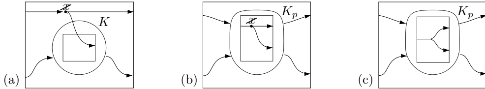
Figure 9: In this sequence of graphs we push name-restriction progressively inside controls until it can be dismissed. We use this technique in defining a combinatoric presentation for symmetric action calculi.
