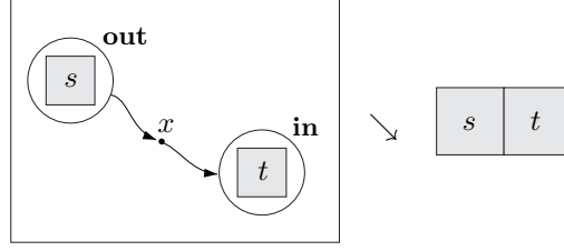
Figure 6: The reaction relation for SPIC.
