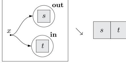
Figure 3: The reaction relation for PIC. The contents of the controls out and in correspond to concretions and abstractions in the \pi -calculus. (We shade s and t to indicate that they are being used as parameters).
