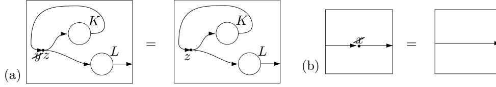
Figure 5: Graph (a) shows an application of the \sigma -axiom corresponding to the symmetric term equation (y^+ \cdot z^- \otimes y^+ \cdot K \cdot z^- \otimes y^+ \cdot L)_y = (z^+ \cdot K \cdot z^- \otimes z^+ \cdot L) . Graph (b) shows the \delta -axiom.
